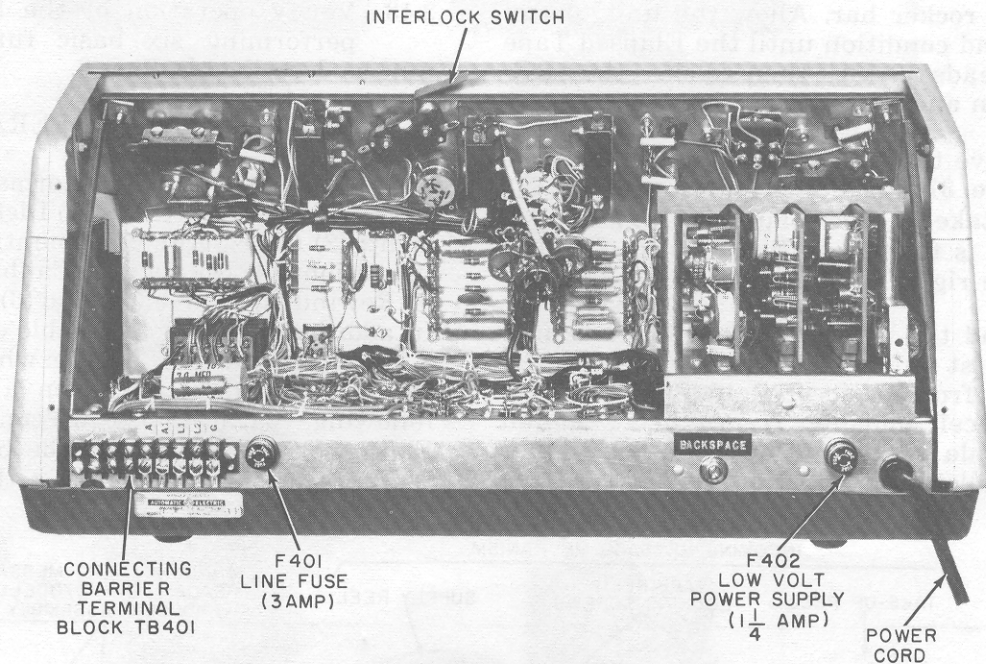
Figure 2. Model RFP (Rear view - back panel removed).
