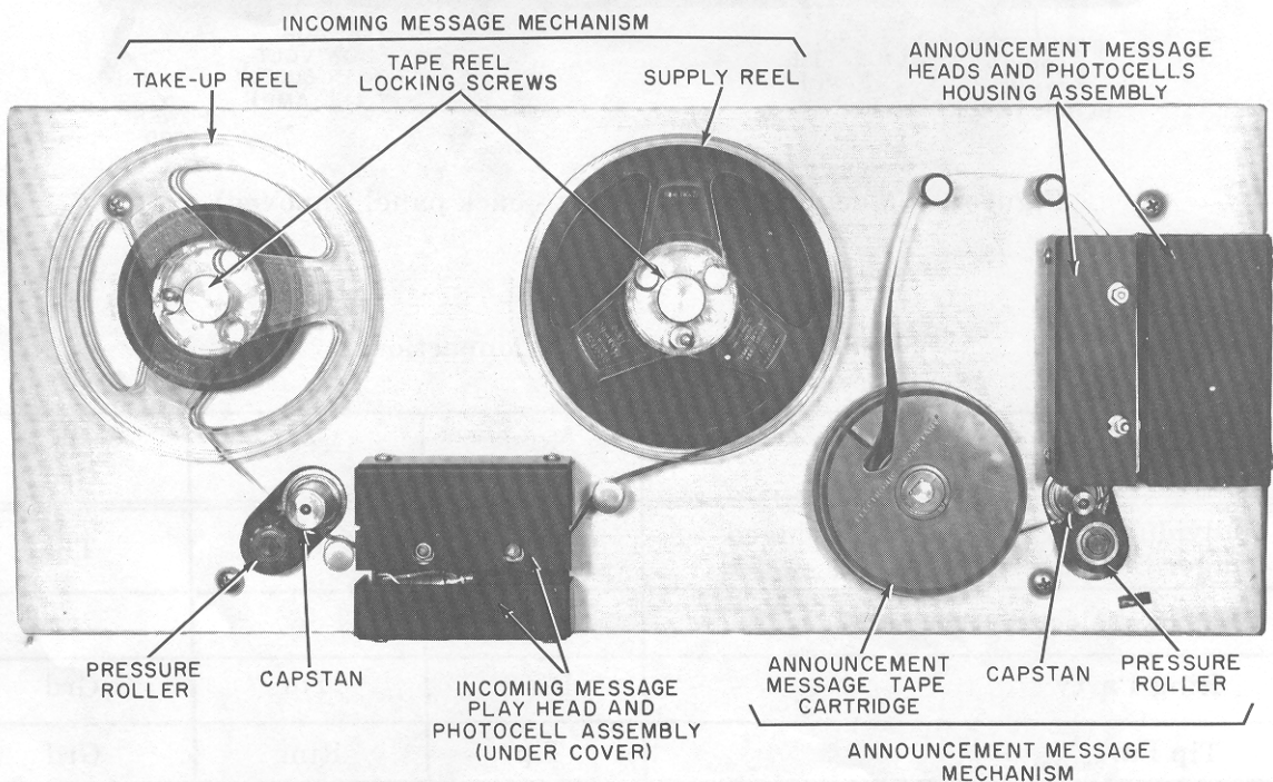
Figure 3. Model RFP Tape Deck (Top view).
