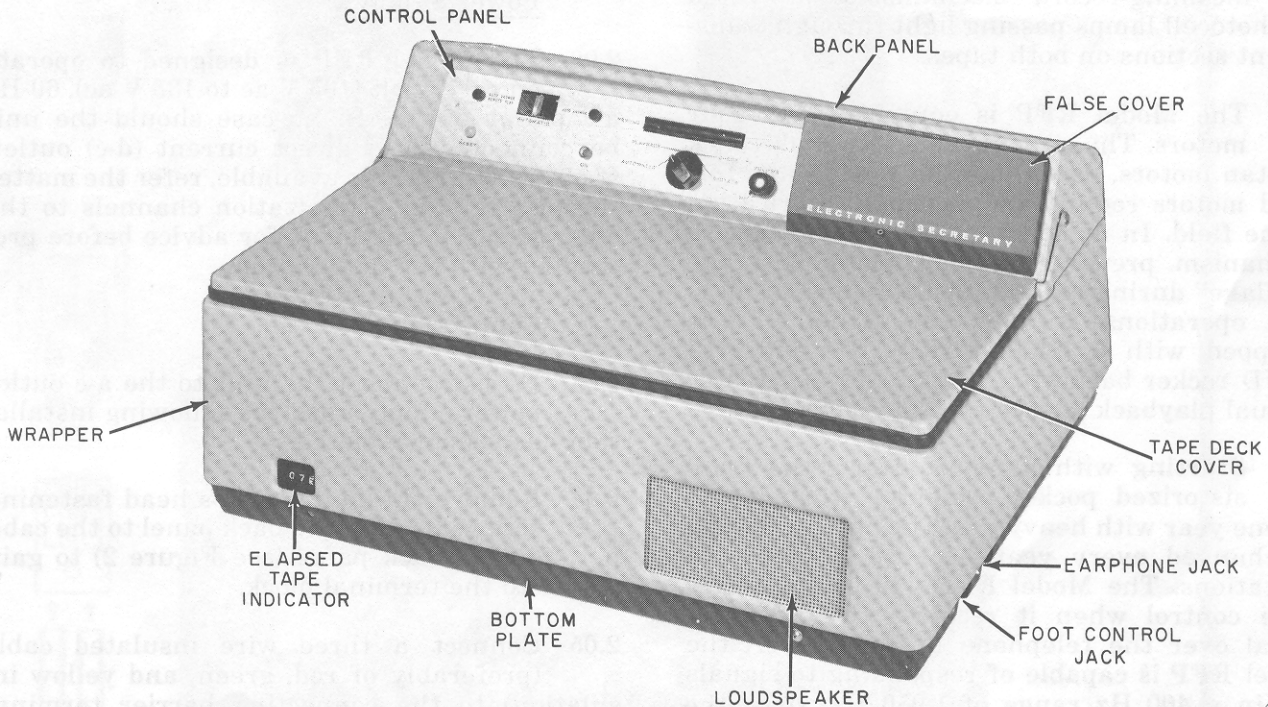
Figure 1. Model RFP (Front view).
