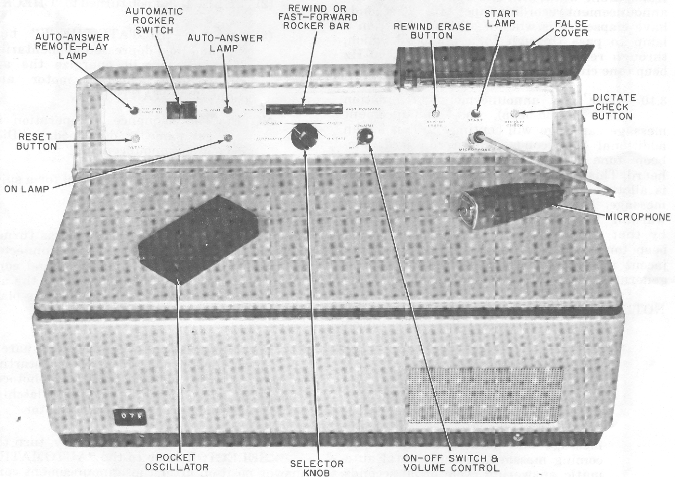
Figure 4. Model RFP - Control Panel.
